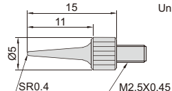
Needle Point
