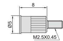
Flat Point
