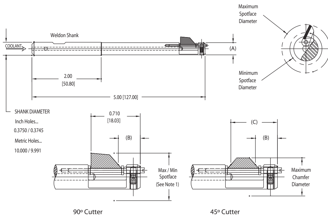
90° Cutter
